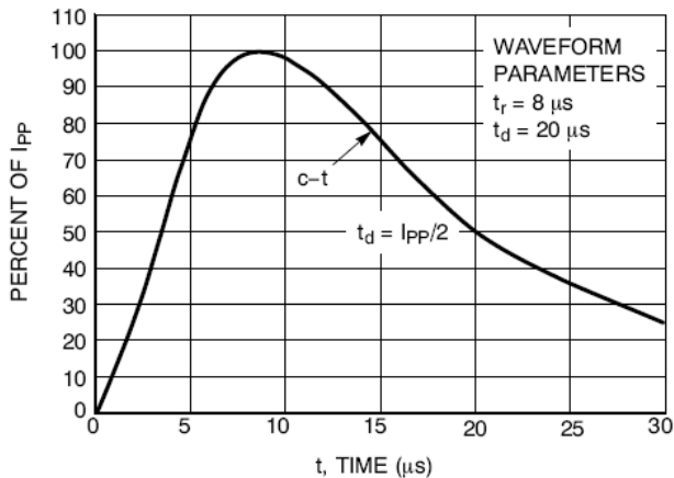
Figure 1. Pulse Waveform
